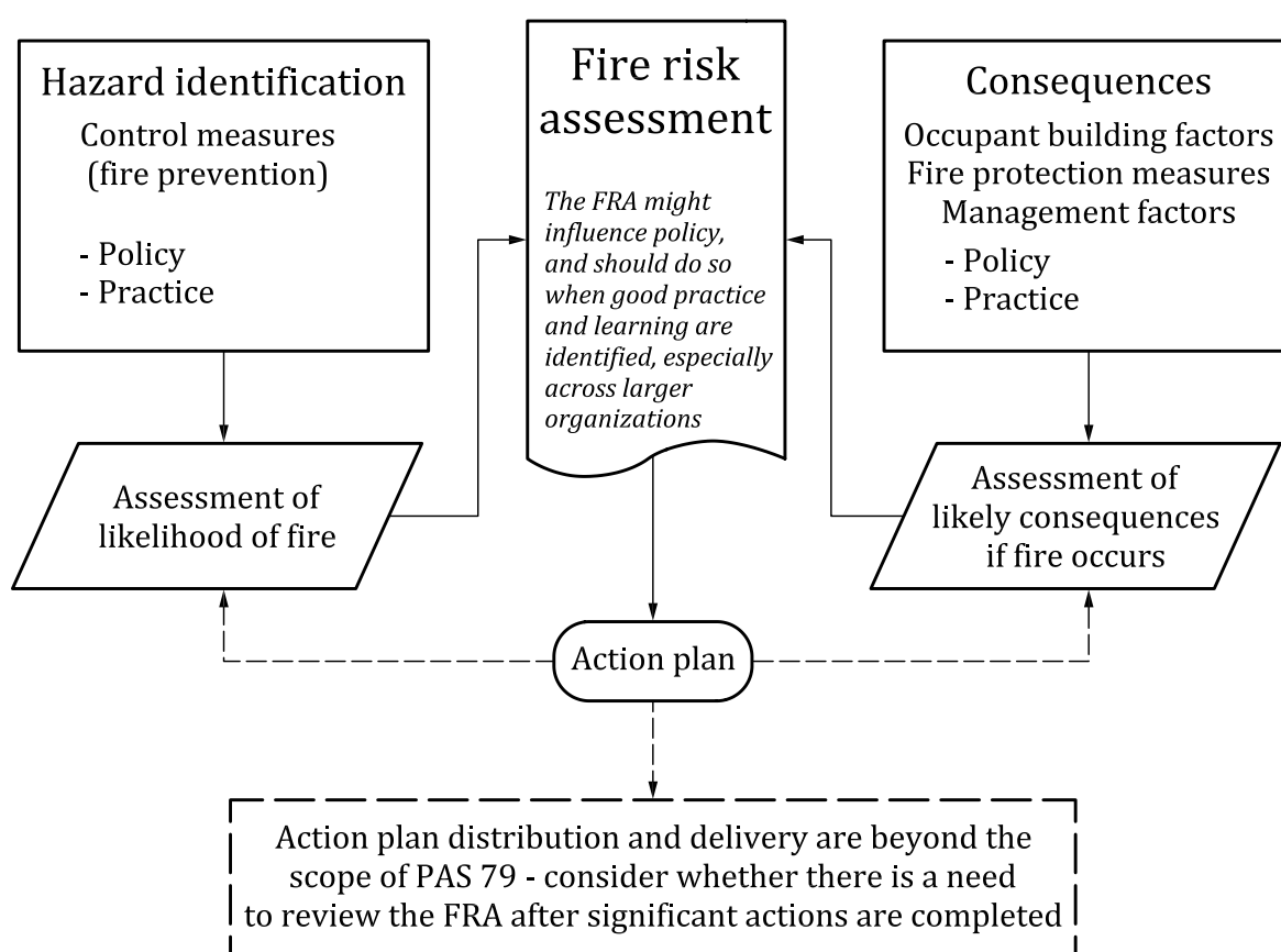
Figure 1 – Schematic of fire risk assessment process
